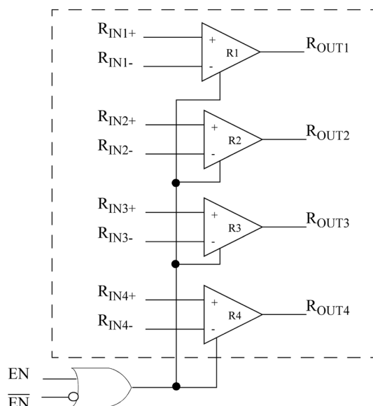
Figure 1. UT54LVDS032 Quad Receiver Block Diagram
