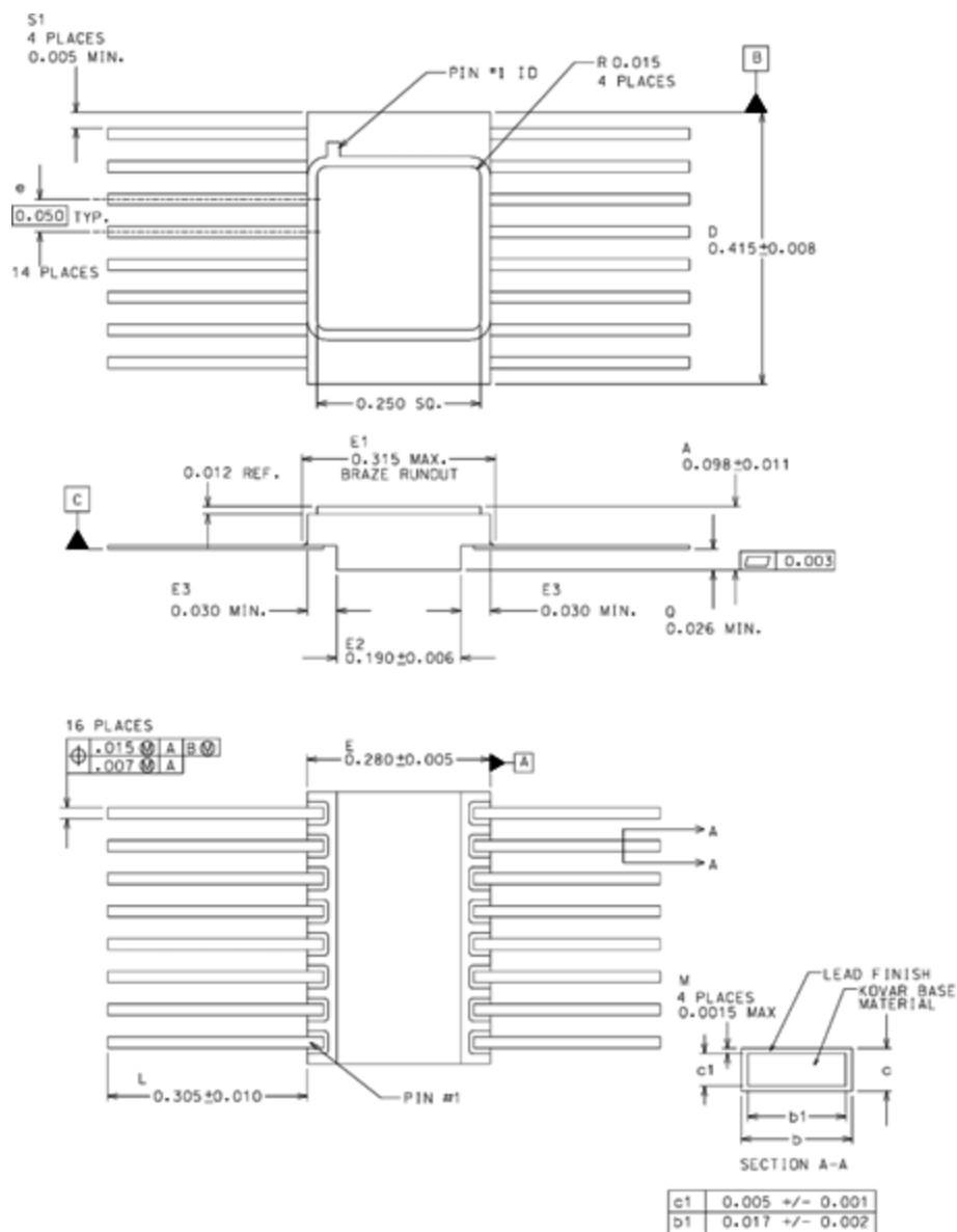
Figure 8: 16-pin Ceramic Flatpack
