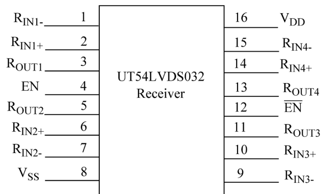
Figure 2. UT54LVDS032 Pinout
