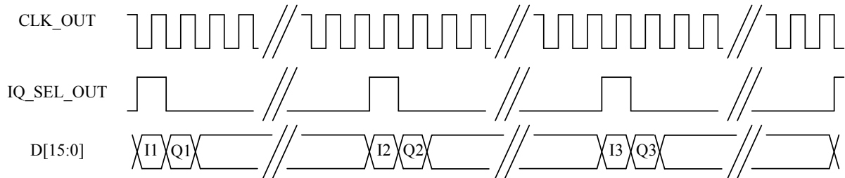
Fig. A-8 DATA timing for CDMA2000 1X
