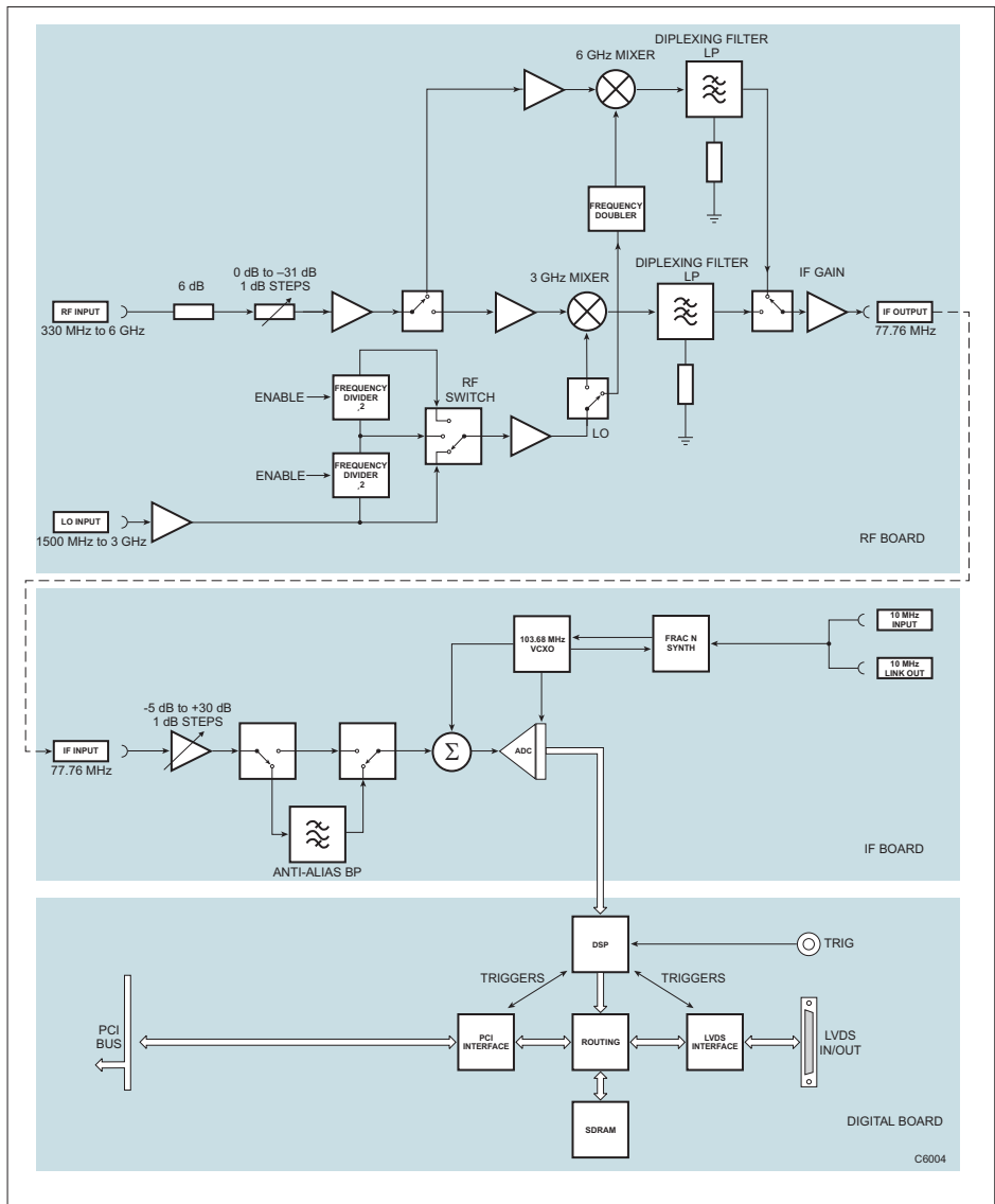
Fig. 4-1 Block schematic diagram
