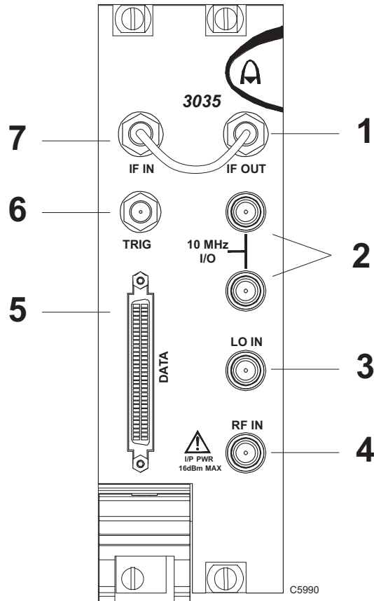
Fig. 3-1 3035 front panel
