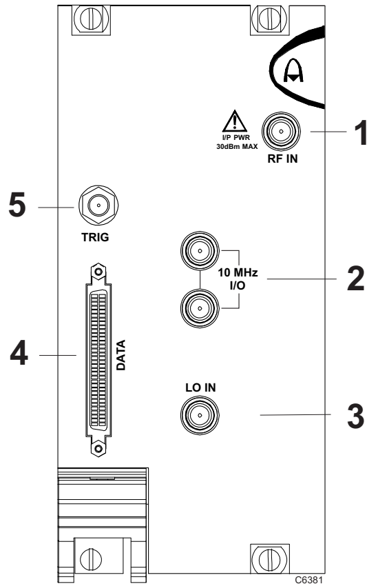
Fig. 4 3035, 3036 front panel
