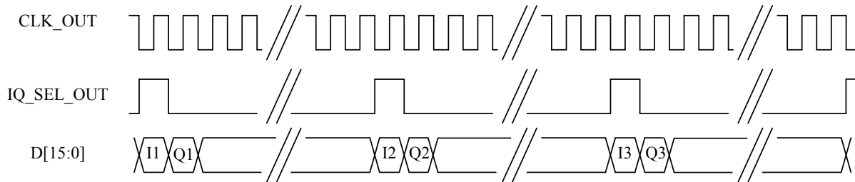
Fig. 29 DATA timing for CDMA2000 1X, 125 MHz clock
