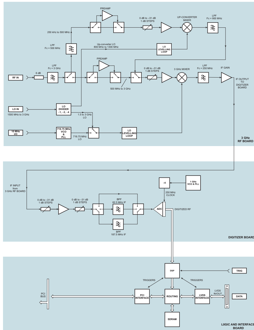
Fig. 34 3030C block schematic diagram
