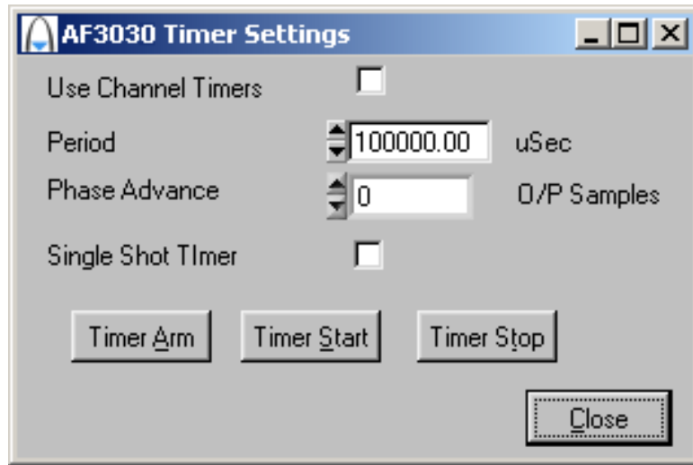
Fig. 3-8 Timer settings
