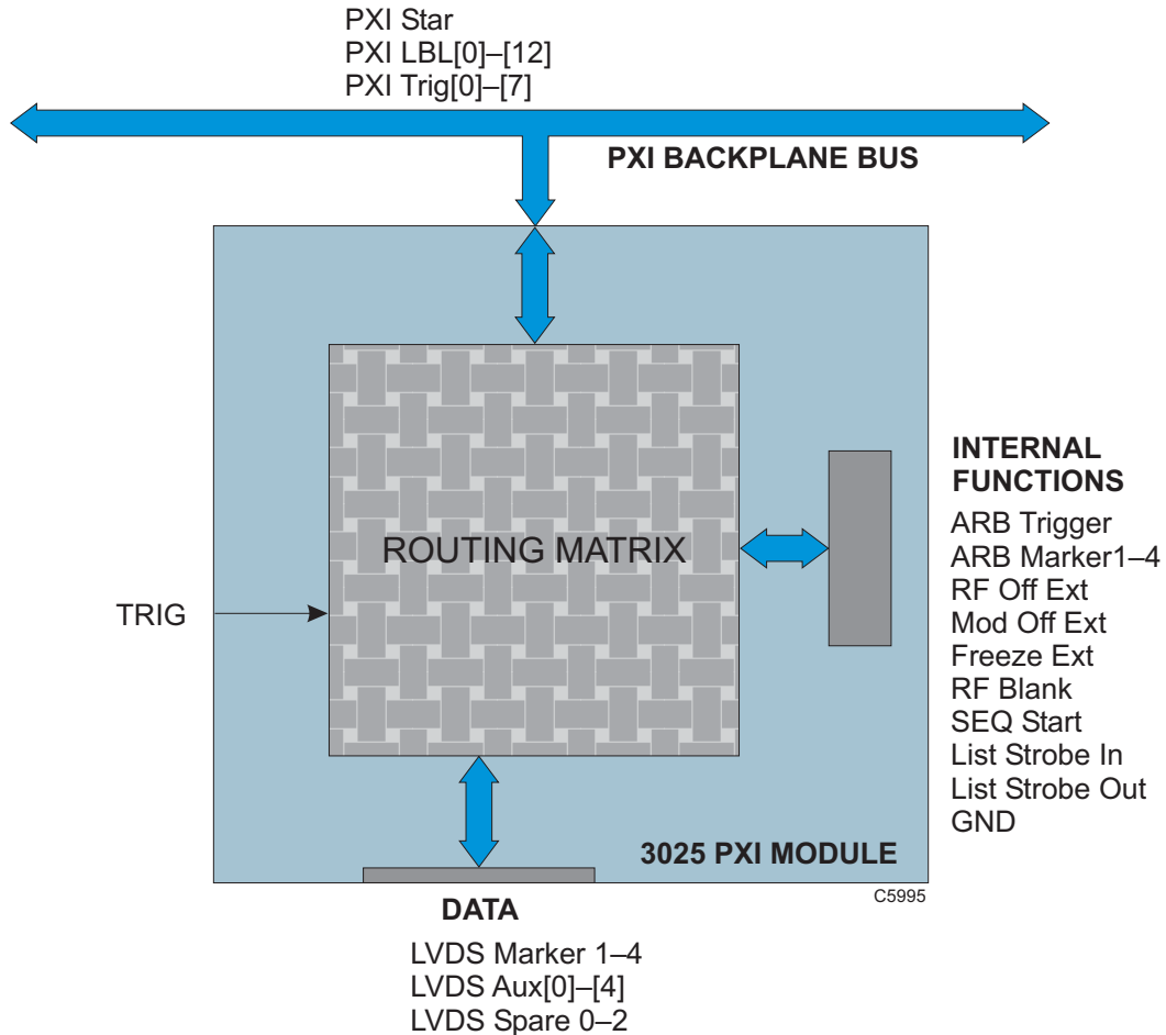
Fig. 3-3 Routing matrix in 3025
