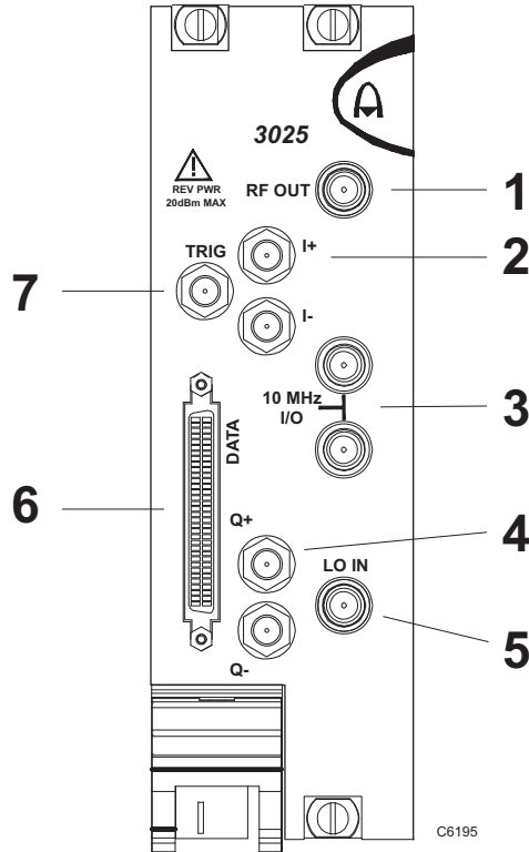
Fig. 3-1 3025 front panel
