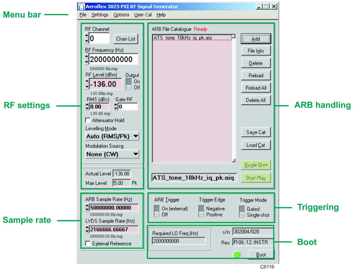
Fig. 3-2 3025 soft front panel
