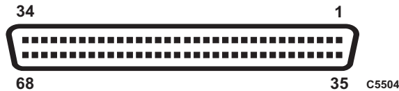
Fig. B-1 DATA connector (looking onto front panel)
