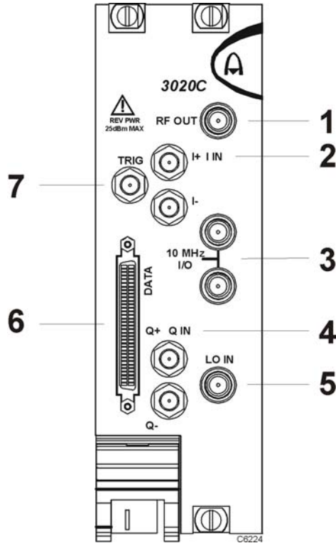
Fig. 3-1 3020C front panel
