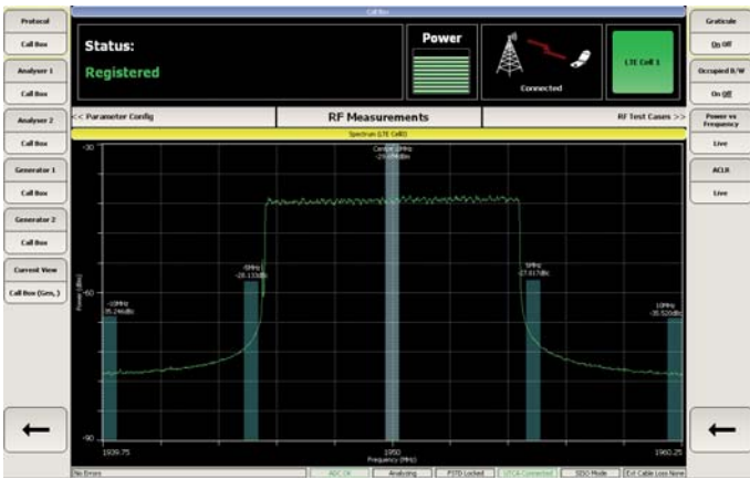
Figure 5. LTE Spectrum and ACLR Measurement
