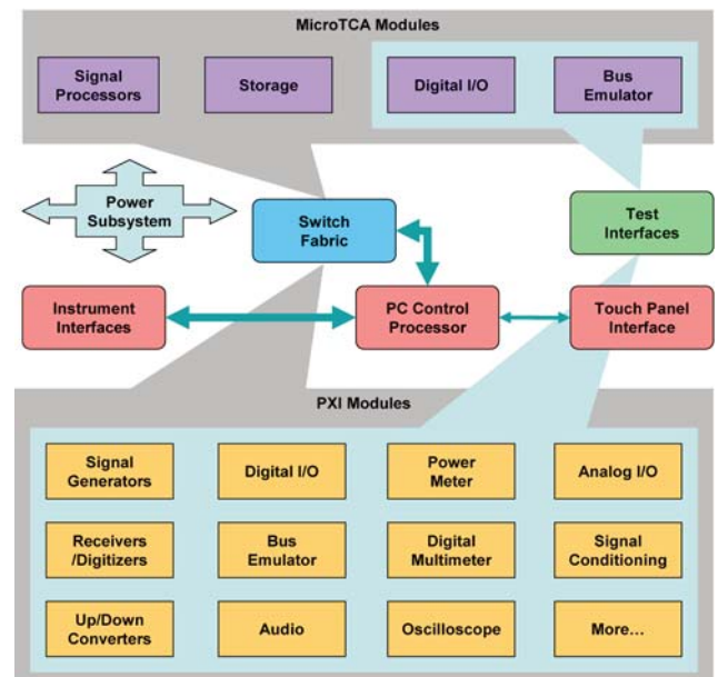
Figure 3 – 7200 Hardware Architecture
