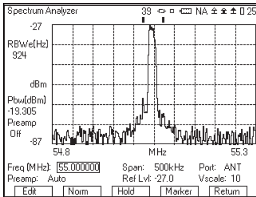
Spectrum Analyzer
