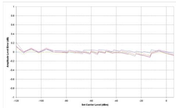
Typical Level Accuracy at 2 GHz (using 3025C)
