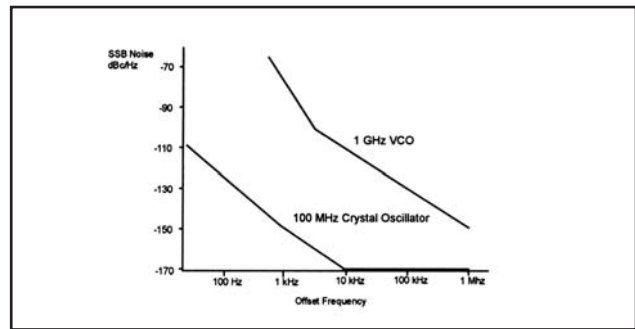
Figure 1 - Typical Oscillator Noise Performance
