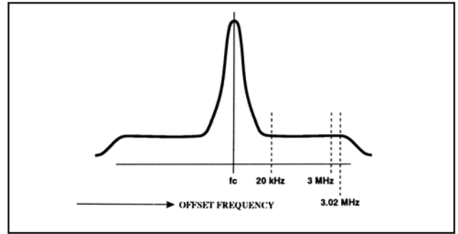
Figure 10 - Effect of noise at the image frequency
