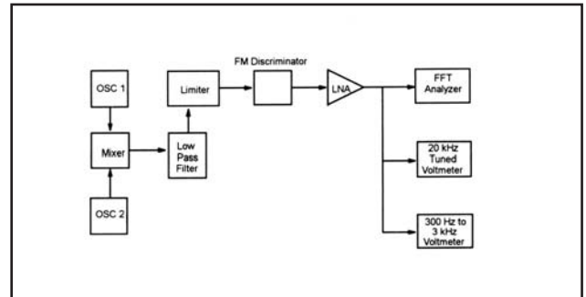
Figure 7 - FM Discriminator Method
