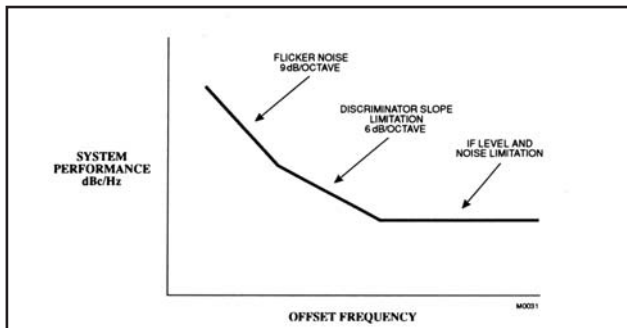
Figure 9 - Performance Limitations of the FM Discriminator Method
