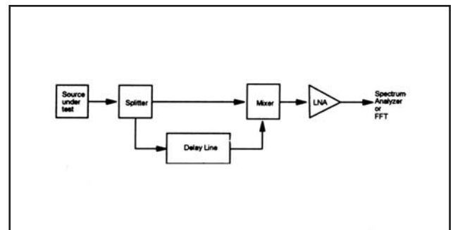
Figure 4 - Delay Line Discriminator
