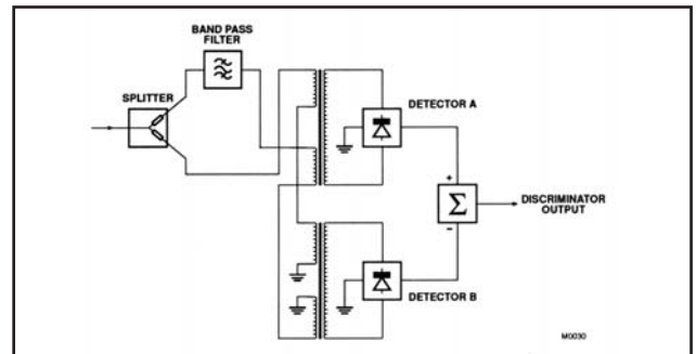
Figure 8 - A High Performance FM Discriminator
