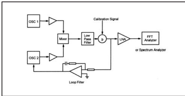
Figure 6 - Measuring the Phase locked Loop effects.
