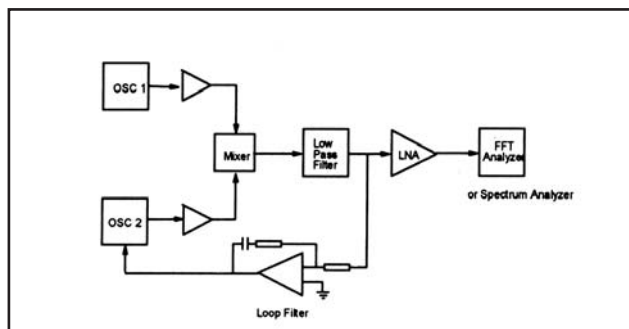
Figure 5 - Quadrature Technique
