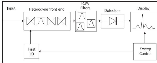
Fig 2 Typical spectrum analyzer architecture.
