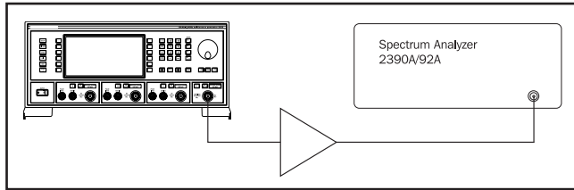
Fig 1 Typical intermod set up using 2026
