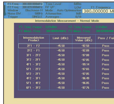
Figure 6. 2309 Intermodulation mode
