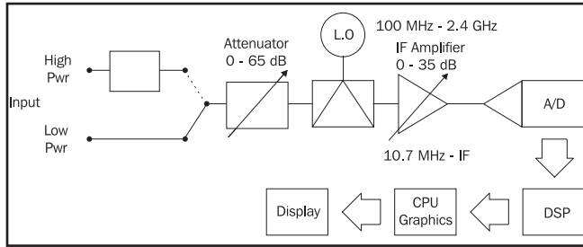
Fig 3 Architecture used in 2309
