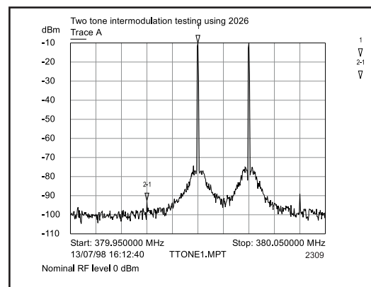
Figure 5. Two tone intermodulation with input at 0 dBm per tone.
