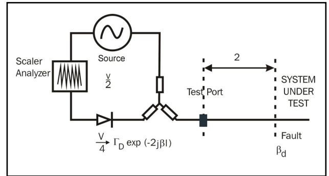
Figure B1 - Phase Encoding Symmetrical power divider
