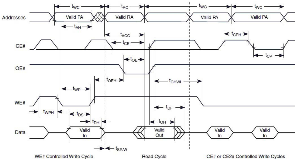
Figure 13. Back-to-Back Read/Write Timings
