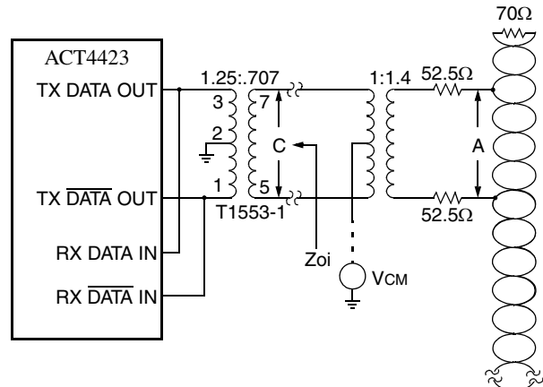
Transformer Coupled Stub
