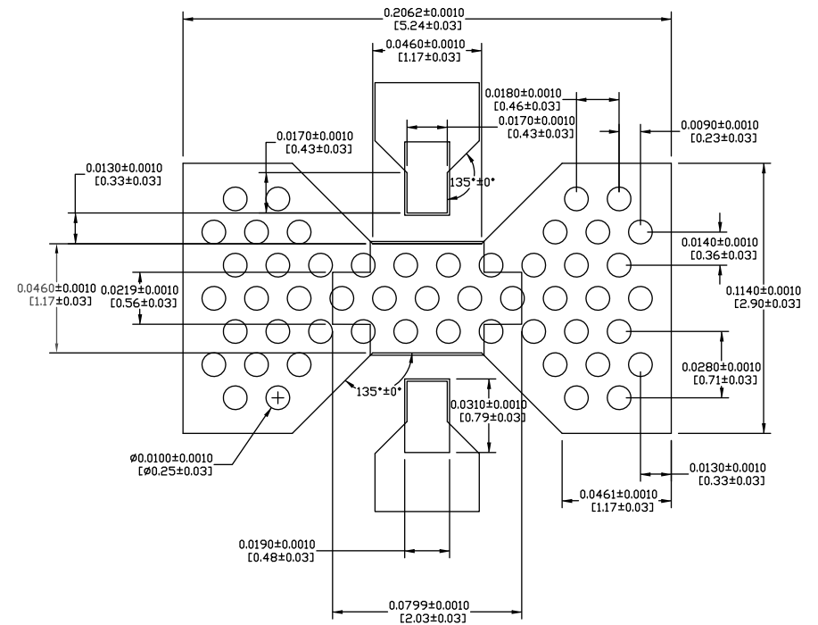
DFN 2615 Package Soldering Footprint
