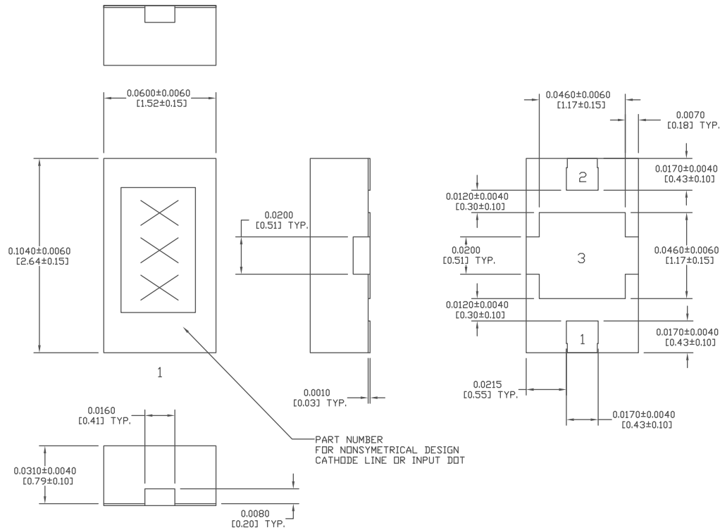
DFN 2615 Package
