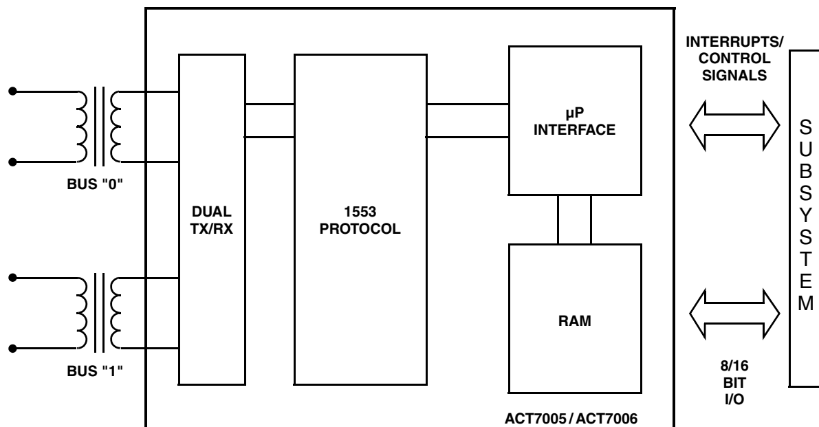
BLOCK DIAGRAM
