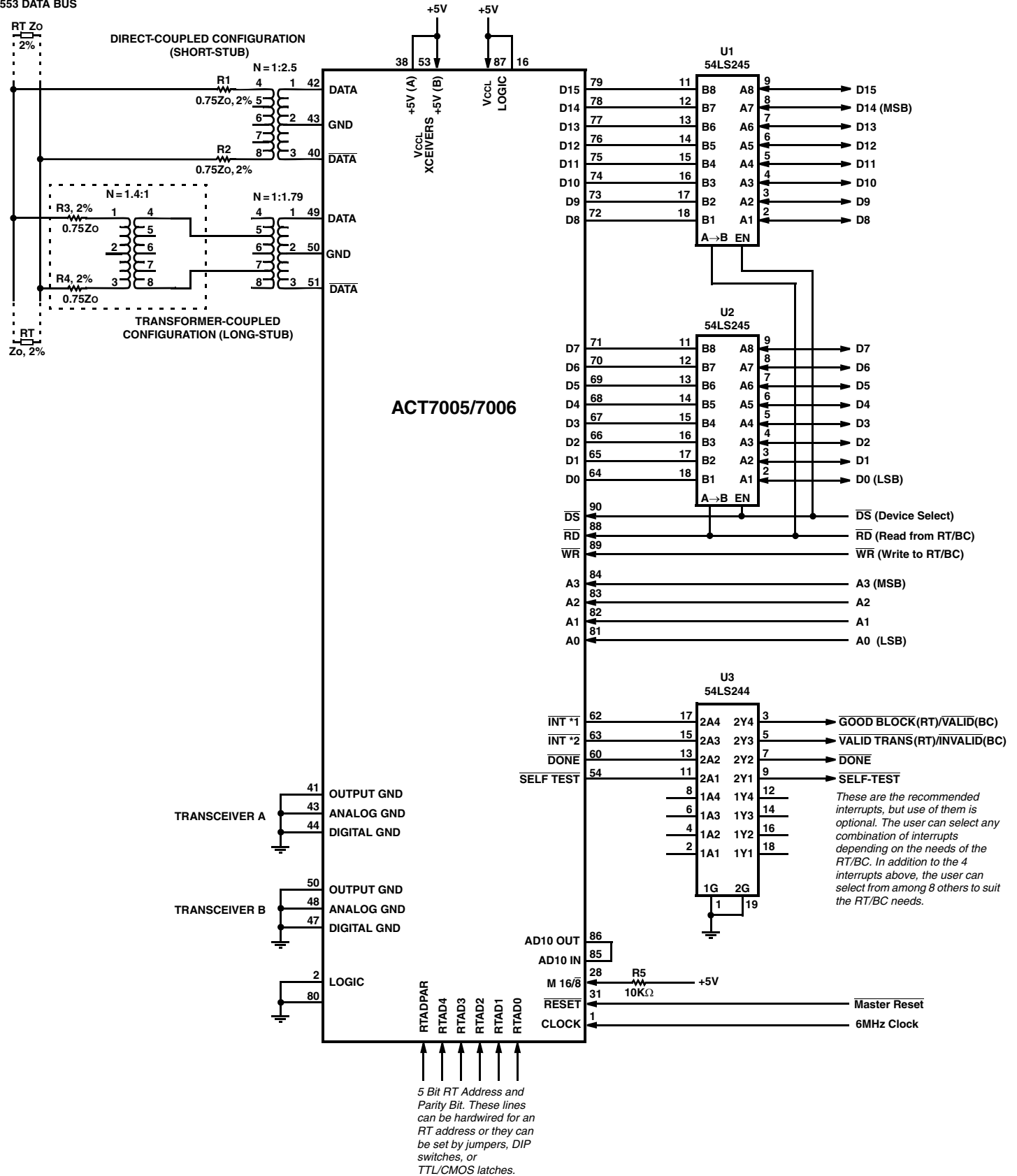
FIGURE 3 – TYPICAL INTERFACE CONNECTIONS
