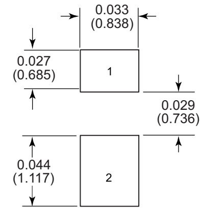
SOLDERING FOOTPRINT
