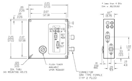
Standard Outline Drawing for Internal Reference & Dual Loop Models up to 18 GHz Note: for frequencies <4 GHz will be 0.82 inches/20.82mm. Note 2: REF MON connector becomes REF IN on dual loop models.
