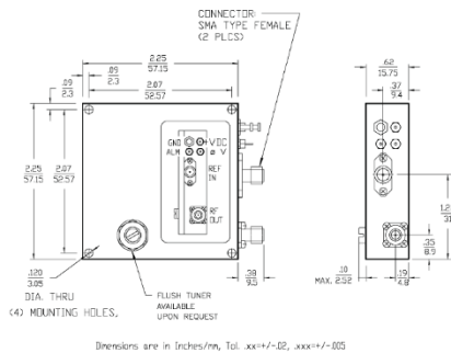
Standard Outline Drawing for Frequencies From 18 GHz to 45 GHz Note: Output connector will be 2.92 mm female for frequencies Above 26 GHz. Note 2: REF IN connector becomes REF MON on internal Reference Models
